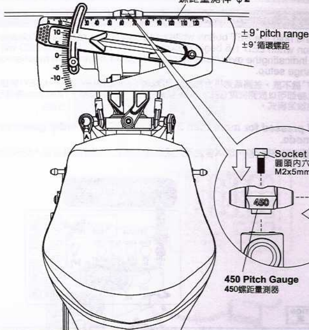
Gauge measuring rod 螺距量測桿 \phi 2
